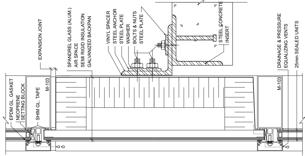
MULLION, CAP & WINDOW WASHING TRACK OPTIONS
