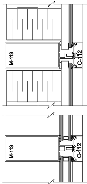
DETAIL 1 NTS
