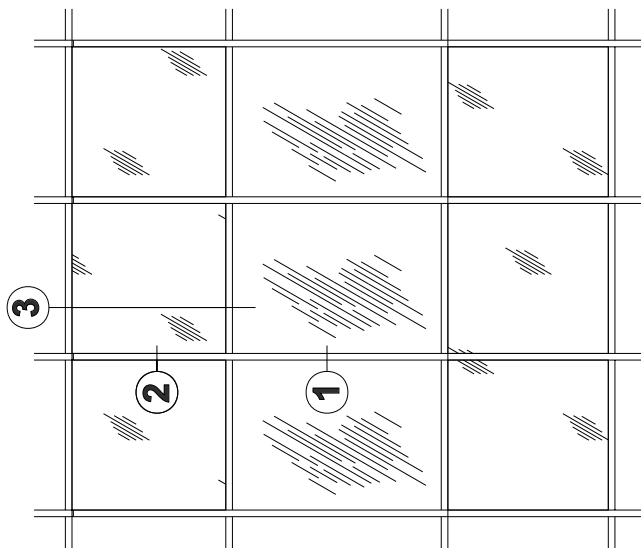
PARTIAL CURTAIN WALL ELEVATION NTS
