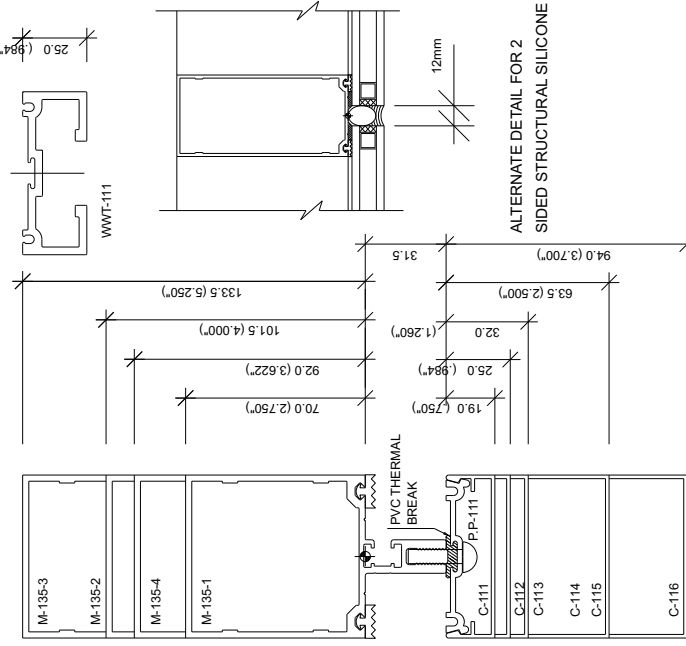
MULLION, CAP & WINDOW WASHING TRACK OPTIONS
