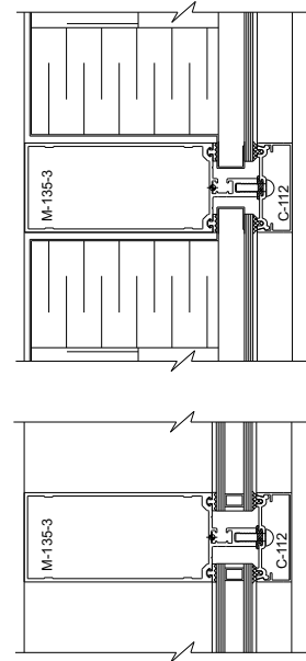
DETAIL 1
