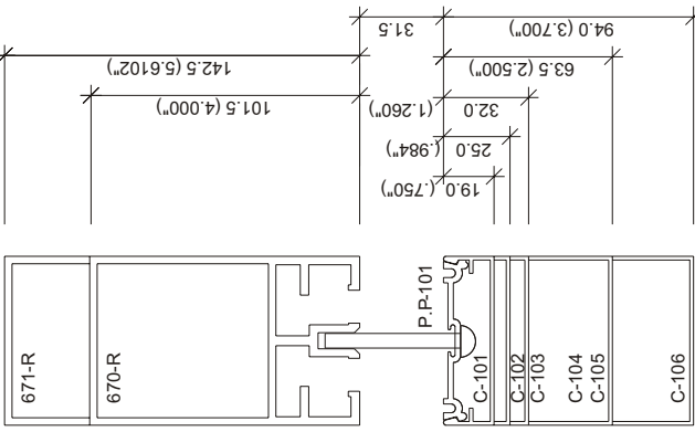
RAFTER, PURLIN, PRESSURE PLATE & CAP OPTIONS SCALE: 1 : 2
