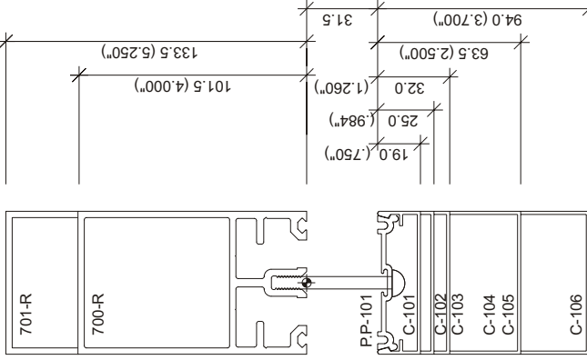
RAFTER, PURLIN, PRESSURE PLATE & CAP OPTIONS
