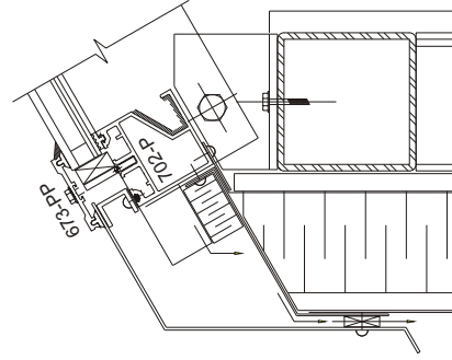
DETAIL 2
