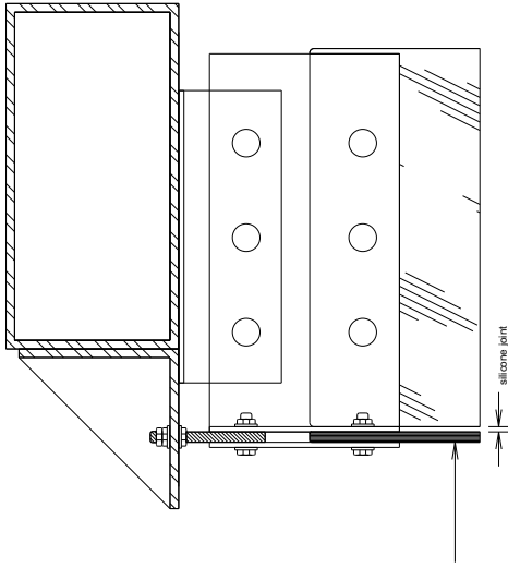
TYP. HEAD DETAIL
