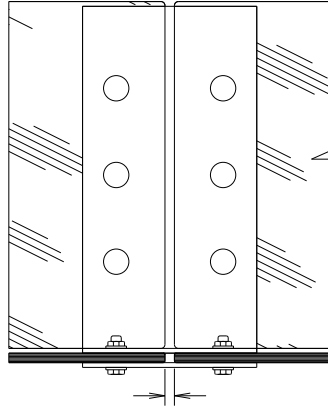
TYPICAL PATCH FITTING
